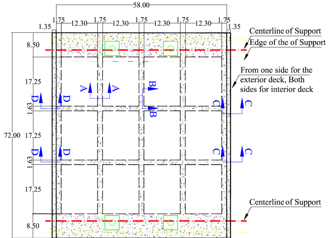
Figure 4.23 Panel 2 (UHPC-HSS)
