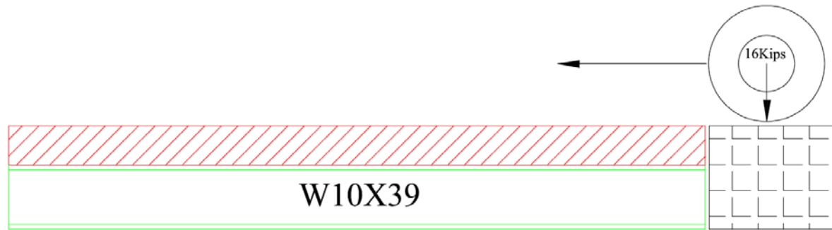
Figure 4.29 Loading Plan
